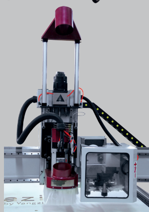
Router 2000x3000 mm -SMART ATC
